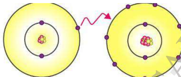
Types of Chemical Bonds – Ionic bonding
