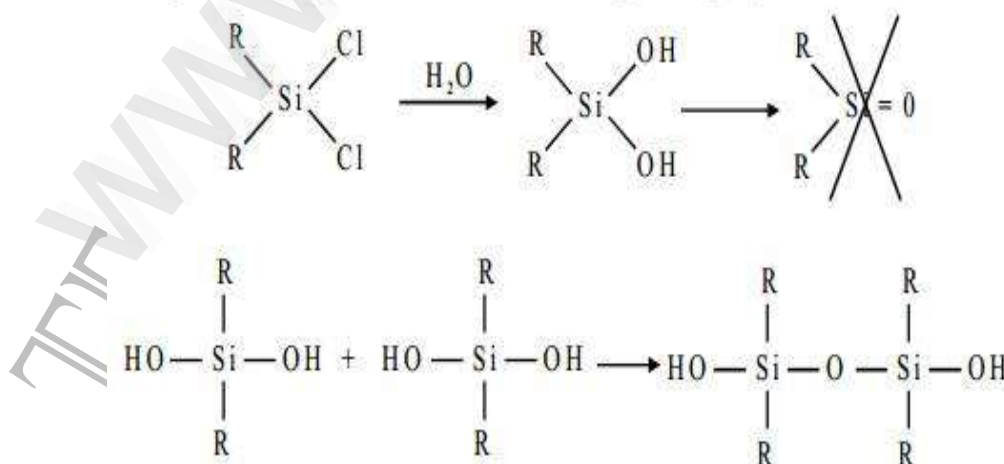
Figure 2: Structure of silicones
