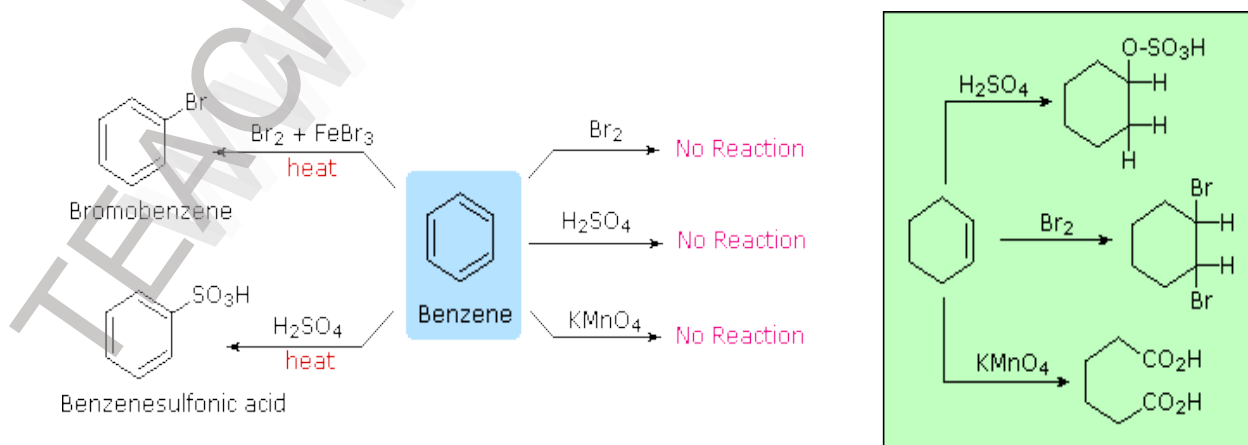
Figure 3: Illustration of addition and substitution reaction with Example
