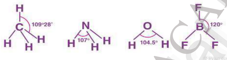
Factors Affecting Bond Enthalpy in Chemical Bonding
