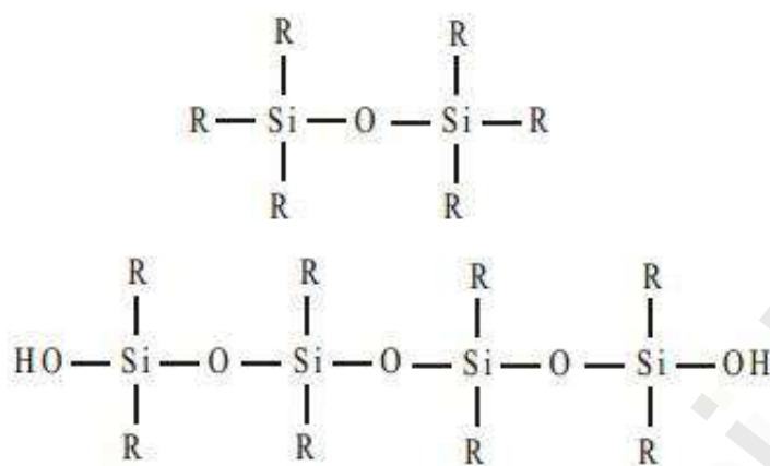
Figure 3: Structure of hexa-alkyl siloxane
