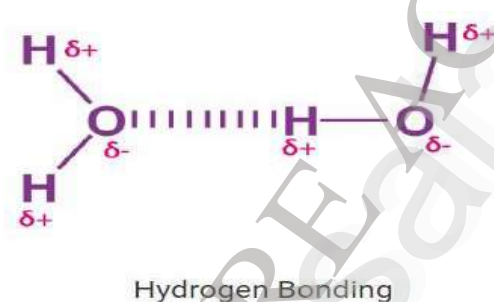
Figure 4: Illustration of Hydrogen Bonding
