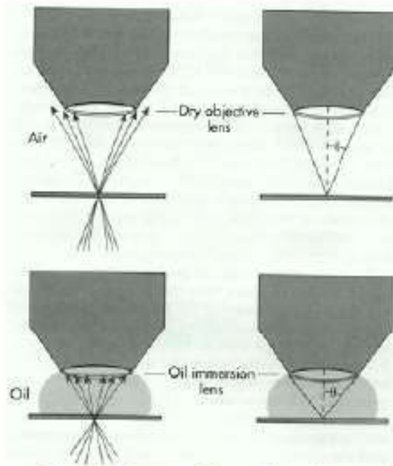
The oil immersion objective and resolution
