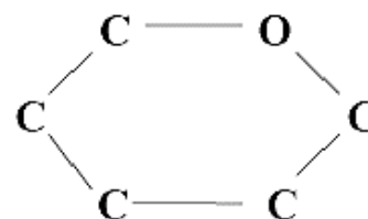
Pyranose Ring
