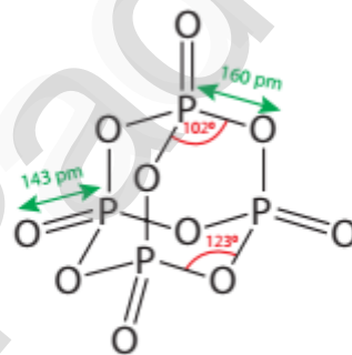
Figure 3.7 Structure of P_4O_{10}
