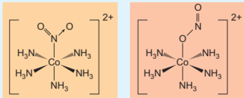
Figure 5.3 Linkage isomers
