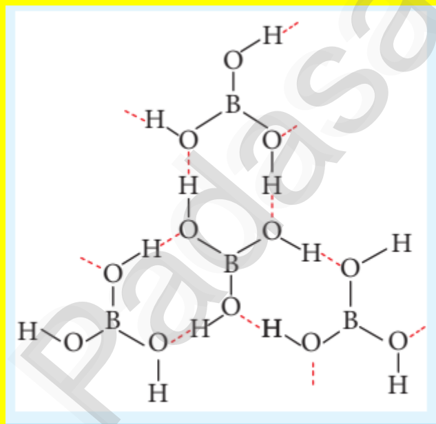
Figure 2.2 Structure of boric acid
