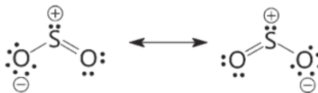
Figure 3.9 Structure of sulphur dioxide.
