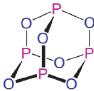
Figure 3.6 Structure of P_4O_6
